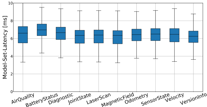
Figure 7: Model-Set-Latency for Runtime properties for the TurtleBot evaluation runs.
