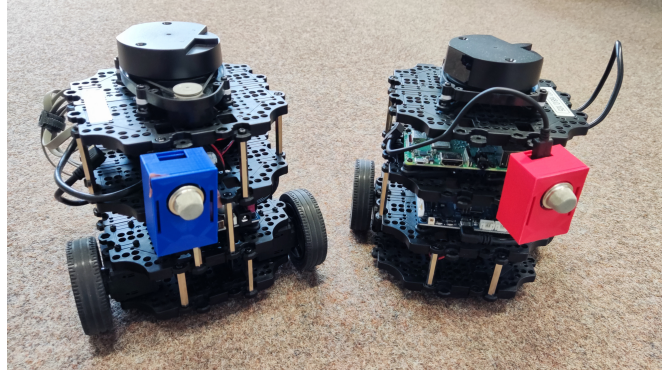
Figure 6: Two of the TurtleBot robots equipped with an additional CO 2 sensor.
