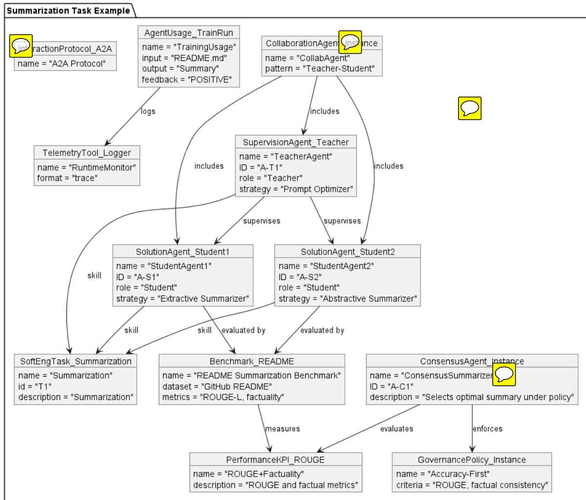
Figure 25: Example of a multi-agent system for summarizing GitHub README files, represented using the MOSAICO taxonomy.
