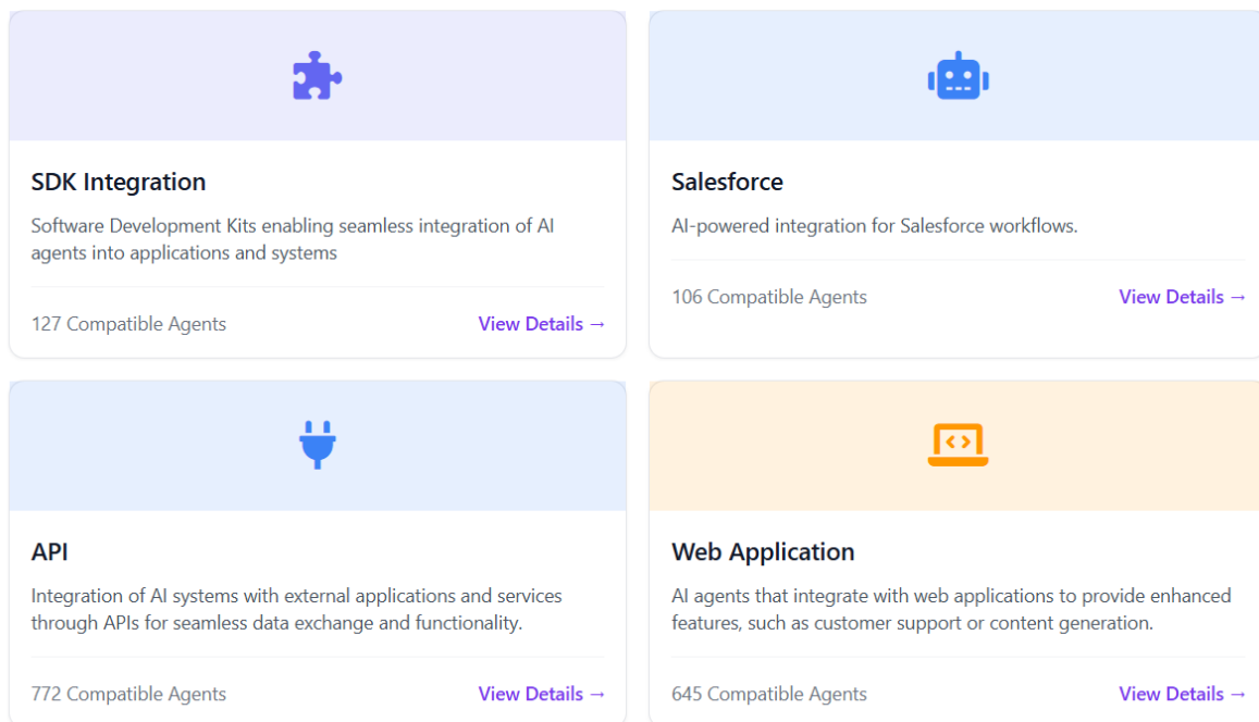
Figure 23: AgentLocker integrations
