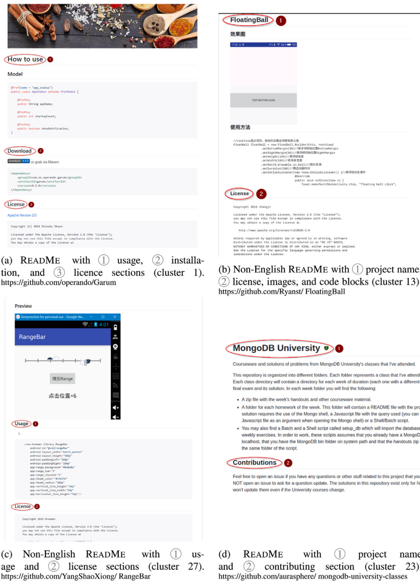
Fig. 2. Example README files from clusters 1, 13, 23, and 27.
