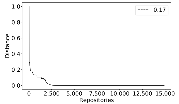
Fig. 4. The k -dist plot: distance graph for our Java repositories. The x -axis is the number of repositories whose k th nearest neighbor is at the distance given on the y -axis. The horizontal line intersecting at distance 0.17 shows the first knee point.
