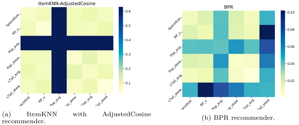
Fig. 5. Choosing the two best DCs on BookCrossing dataset for two RSs: ItemKNN (left) and BPR (right).
