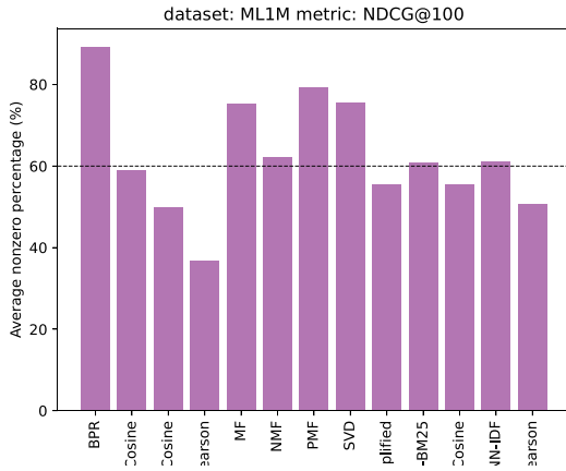
(a) ML-1M on NDCG@100.
