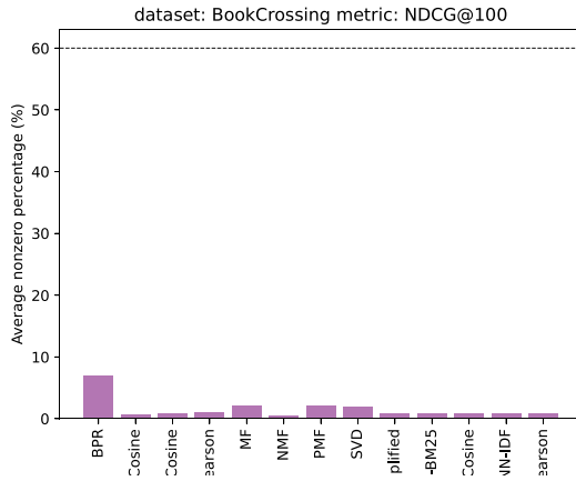
(c) BookCrossing on NDCG@100.
