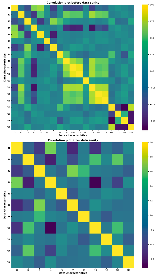
Fig. 2. Correlation plot of the data characteristics in ML-1M before (top) and after (bottom) data sanity check. Note that higher correlation values are harmful for the regression model estimation. Note also that the square clusters on the top figure occur when aggregating a certain feature over users via different statistical aggregation functions (e.g., mean, std, skewness, kurtosis).
