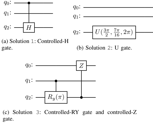
Fig. 7: Optimal oracle solutions obtained through NSGA-III.
