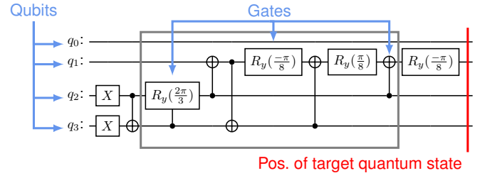
Fig. 1: Example parameterized quantum circuit; red line: position of produced quantum state
