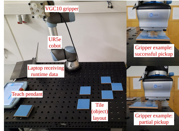
Figure 1: Experimental setup including a UR5e cobot from UR equipped with an OnRobot VGC10 vacuum gripper, displayed with the tiles acting as the objects to be moved around. Explanatory text in red.
