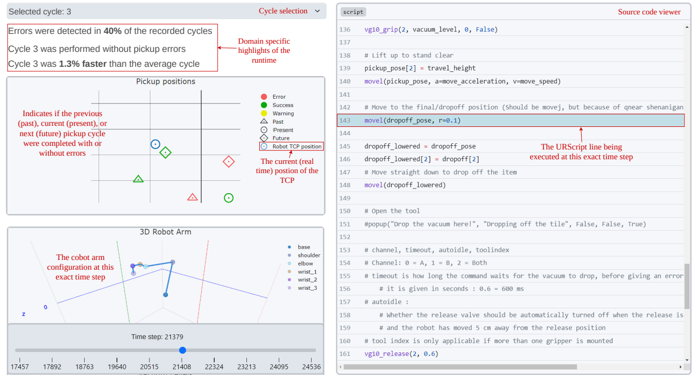
Figure 2: The view of our debugging visualization tool. Explanatory text in red.
