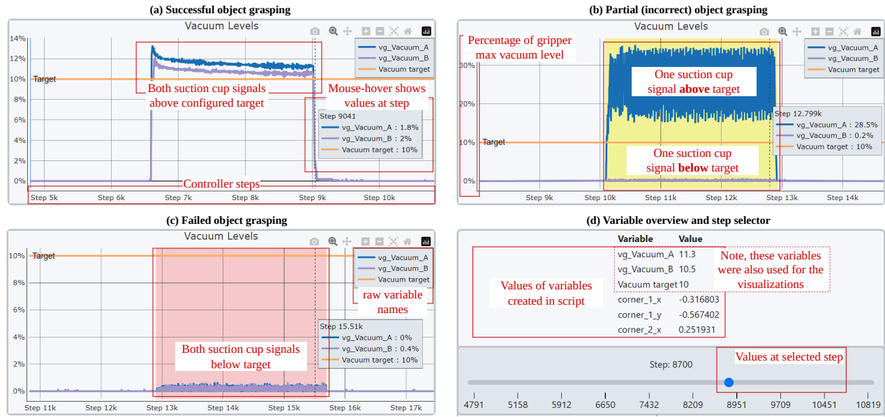
Figure 3: Vacuum level visualization for success, fail and partial grasping. Explanatory text in red.
