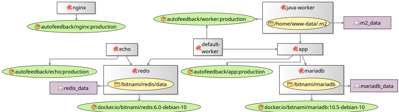
Figure 3: Example containers model, based on the AutoFeedback open-source system
