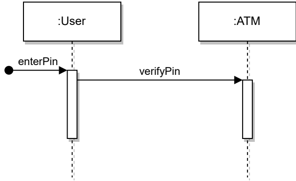
Figure 3. Sequence Diagram of ATM
