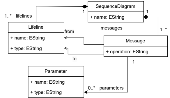
Figure 2. An excerpt of the Sequence Diagram metamodel
