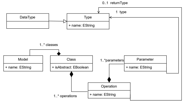
Figure 1. An excerpt of the Class Diagram metamodel
