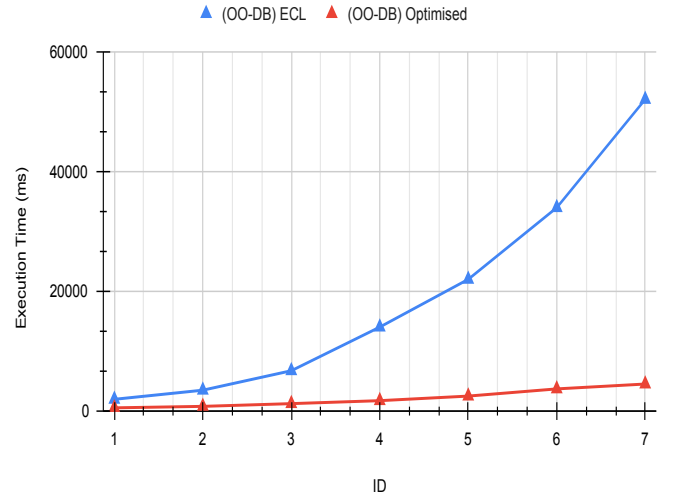
Figure 7. Comparison of Execution time in OO DB Comparison
