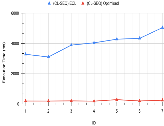
Figure 8. Comparison of Execution time in Class Sequence Diagram Comparison
